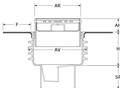
Technical drawing
